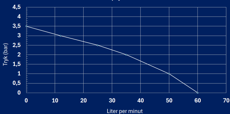
Pumpeydelse
